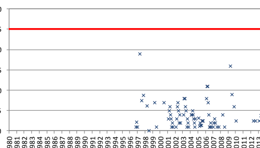
ES030MSPF0613010. Est: TA62708003. Nitratos
