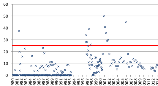
ES030MSPF0427021. Est: TA55905003. Nitratos
