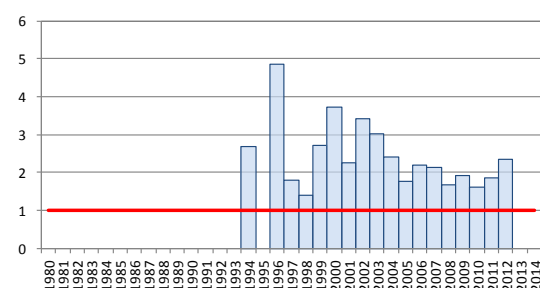
ES030MSPF0628021. Est: TA63002001. Fósforo total. Media anual
