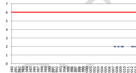
ES030MSPF0736010. Est: TA57909003. DBO5
