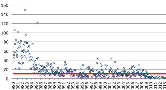
ES030MSPF0416021. Est: TA60505003. DBO5
