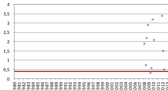
ES030MSPF0519010. Est: TA55807001. Fósforo total
