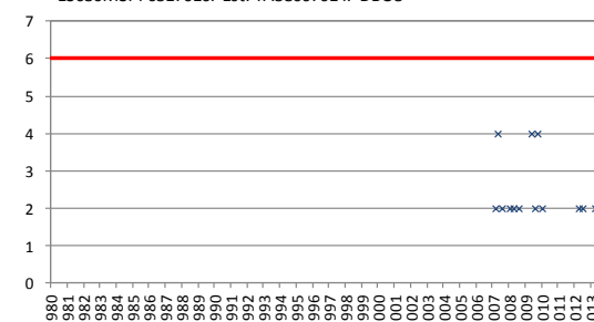
ES030MSPF0517010. Est: TA58007014. DBO5
