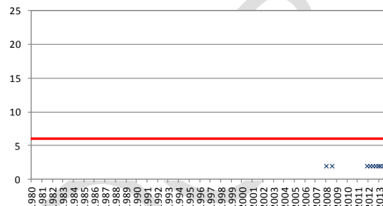
ES030MSPF0912010. Est: TA62210003. DBO5
