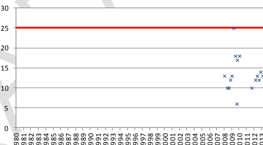
ES030MSPF0118010. Est: TA56102001. Nitratos
