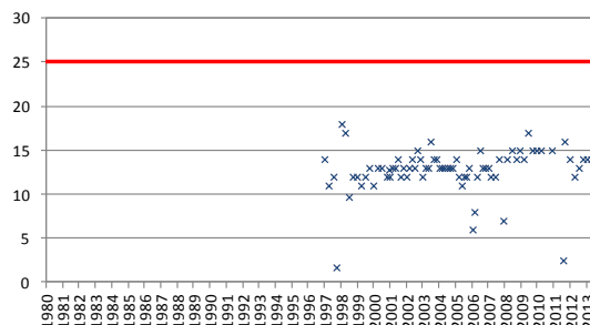
ES030MSPF0128010. Est: TA51501001. Nitratos
