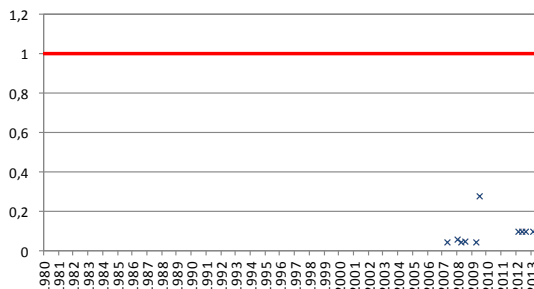
ES030MSPF1030010. Est: TA67514005. Amonio
