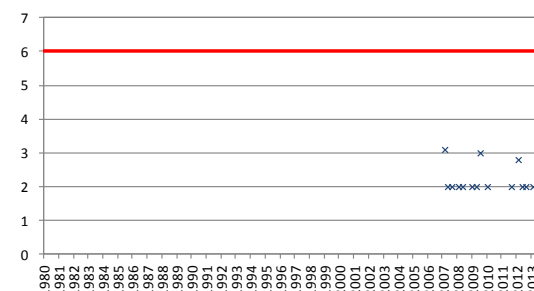
ES030MSPF0405010. Est: TA50806004. DBO5
