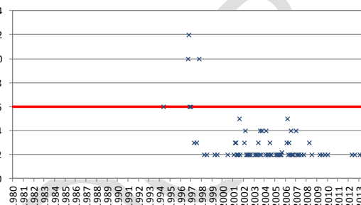
ES030MSPF0613010. Est: TA62708003. DBO5
