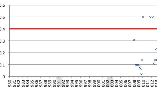
ES030MSPF0118010. Est: TA56102001. Fósforo total
