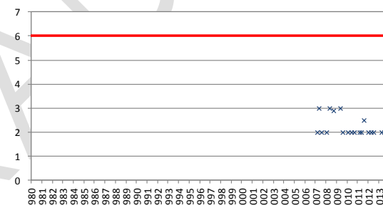
ES030MSPF0614010. Est: TA62708007. DBO5
