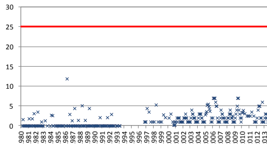
ES030MSPF0507020. Est: TA58007012. Nitratos
