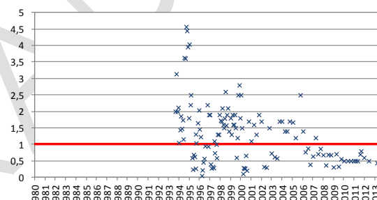
ES030MSPF0419010. Est: TA56005001. Fósforo total
