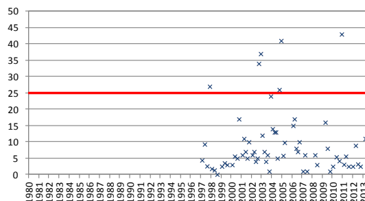
ES030MSPF0518010. Est: TA58007003. Nitratos
