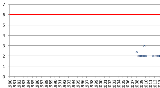
ES030MSPF0118010. Est: TA56102001. DBO5
