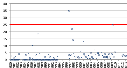
ES030MSPF0706010. Est: TA60109004. Nitratos
