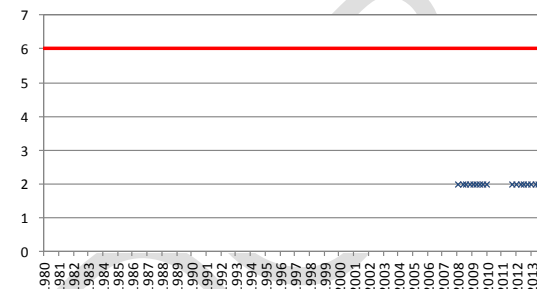
ES030MSPF0721010. Est: TA60009098. DBO5
