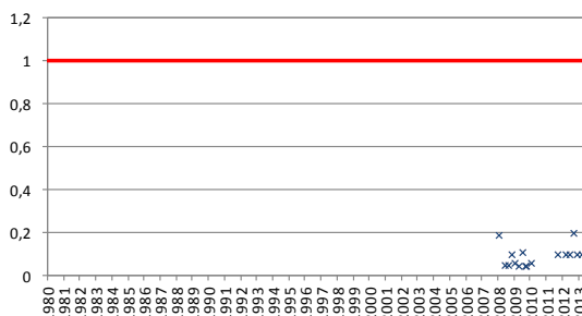
ES030MSPF0118010. Est: TA56102001. Amonio
