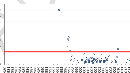
ES030MSPF0613010. Est: TA62708003. Fósforo total
