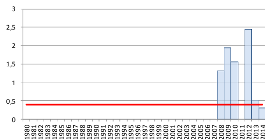
ES030MSPF0519010. Est: TA55807001. Fósforo total. Media anual
